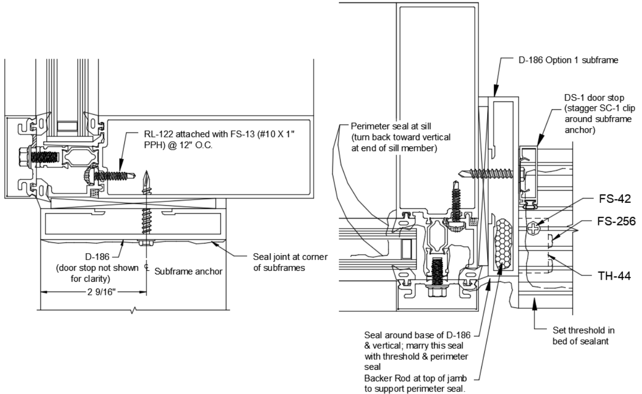
Figure 78: Door Assembly Guide
