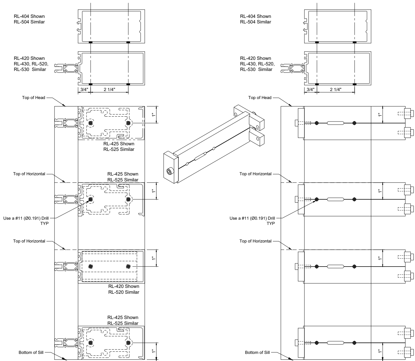
Figure 6: Vertical Mullion Fabrication
