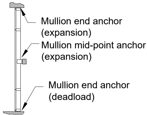
Figure 3: Twin Span
