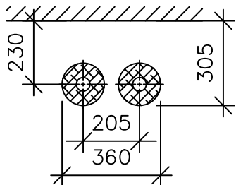
DN40
